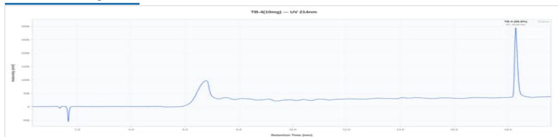
Representative chromatogram, Dedicated V0 (99.76% purity, closest to batch mean of 99.72%)
