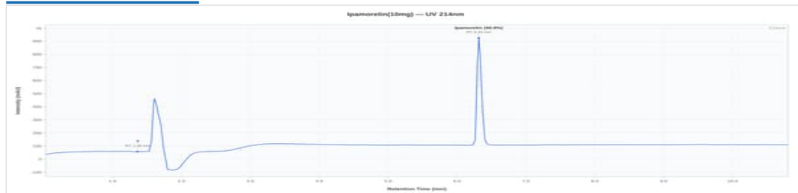
Representative chromatogram, Conformity V1 (100.00% purity, closest to batch mean of 99.93%)
